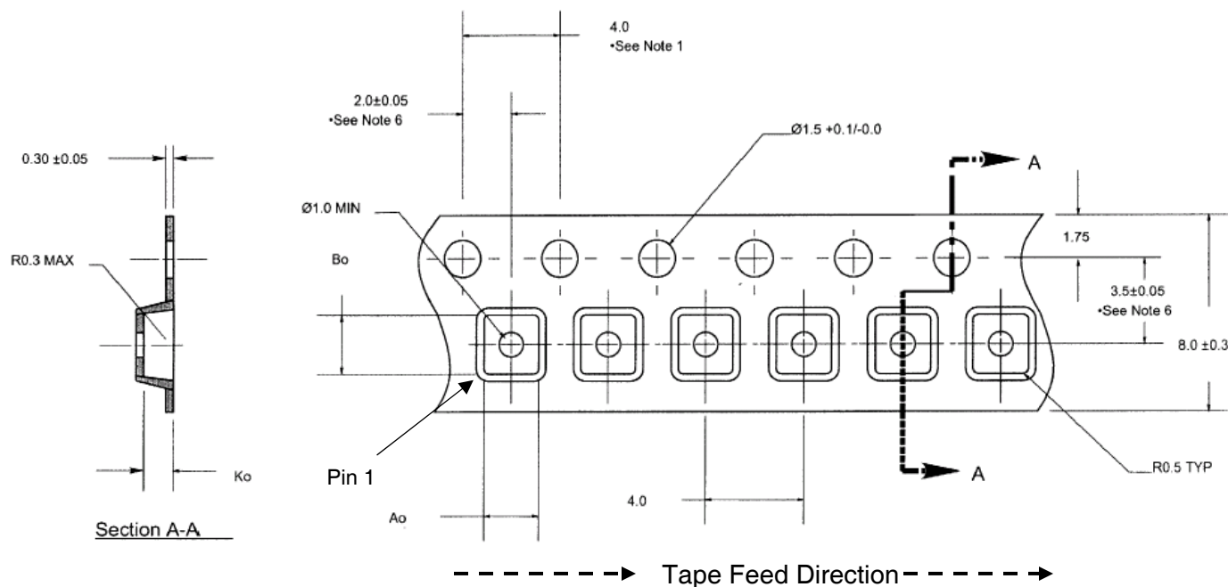
Figure 21. Tape and Reel Specifications
